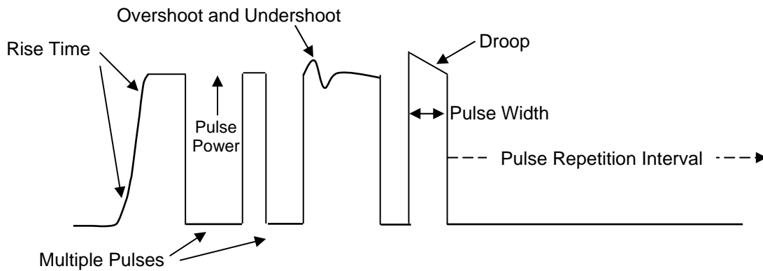
Figure 3. Important time domain characteristics of radar signals.
