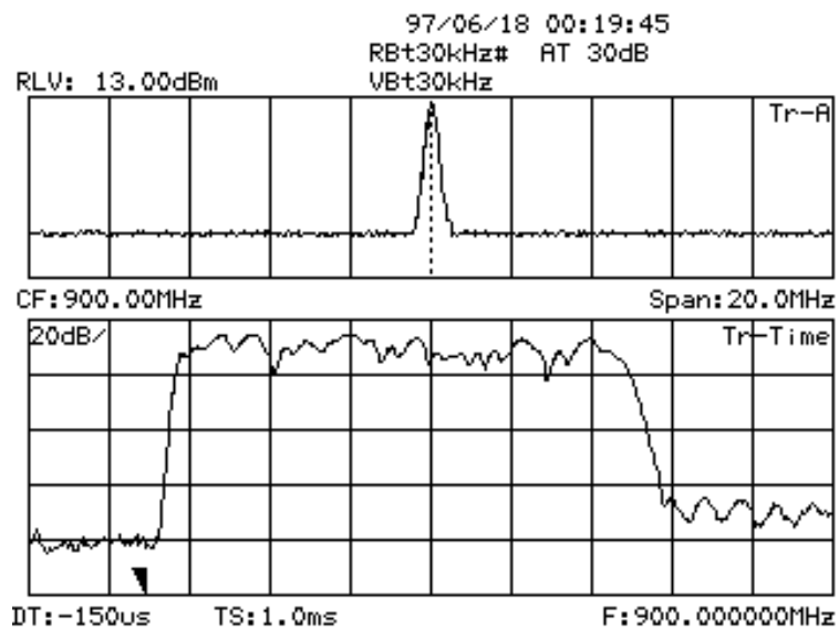
Figure 6. Split-screen frequency domain and time domain displays.
