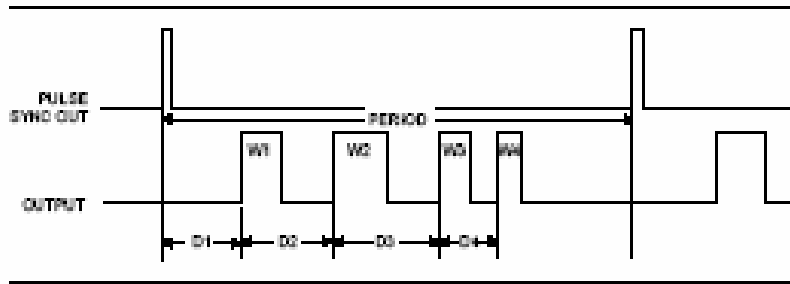
Figure 5. Quad pulse with spectrum analyzer trigger signal.
