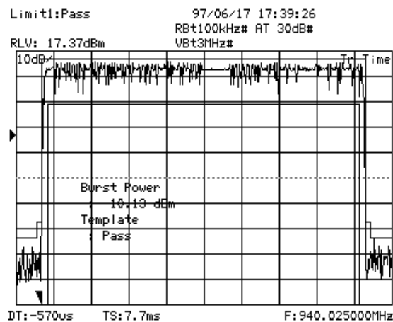
Figure 2. Burst Power in a MS2667C/68C time domain display.
