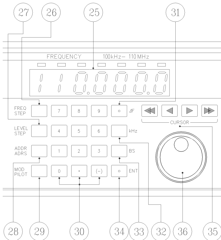
Fig 3.3 Front Panel
