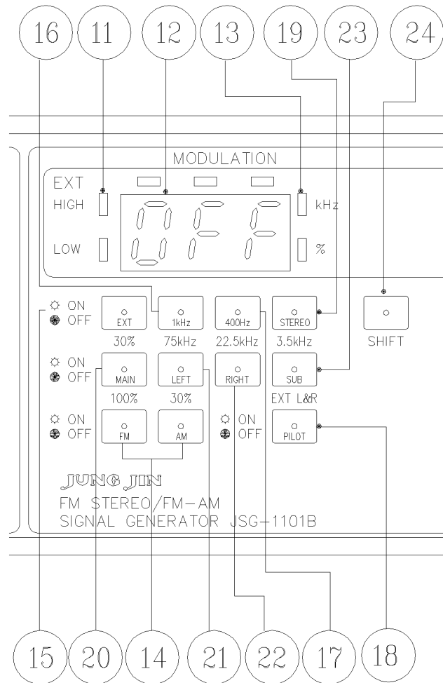
Fig 3.2 Front Panel
