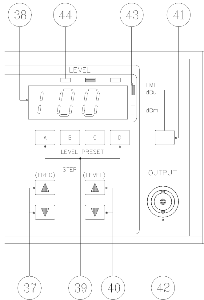
Fig 3.4 Front Panel
