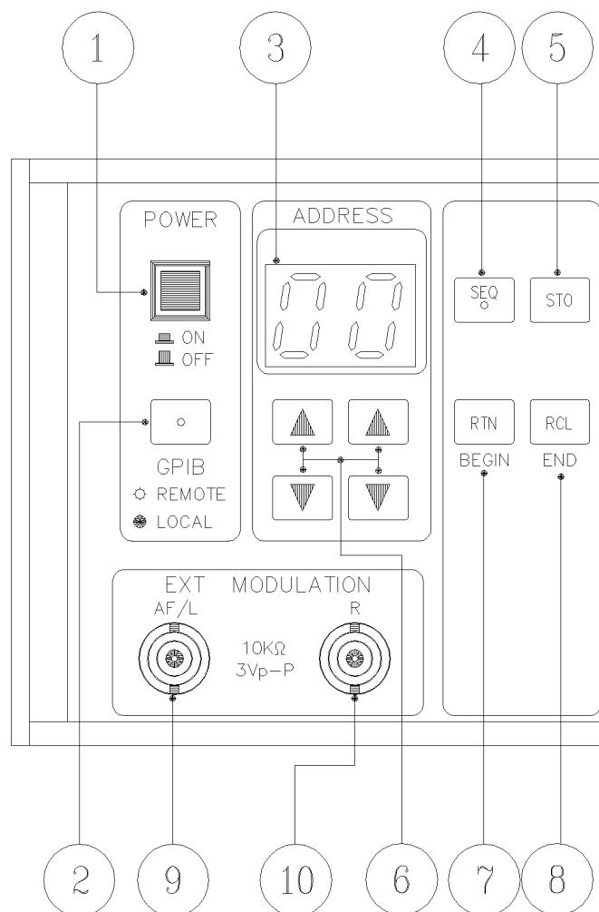
Fig 3.1 Front Panel
