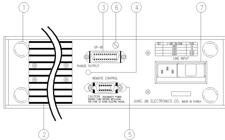
Fig 3.5 Rear Panel
