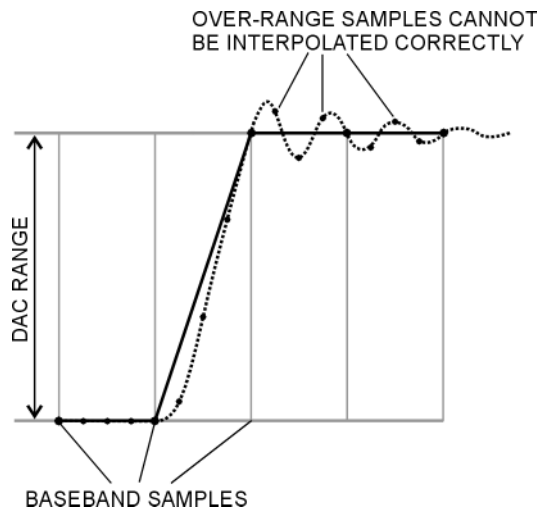
Figure 3-18 Waveform Overshoot
