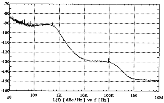
fc = 2 GHz (CW, standard instrument)
