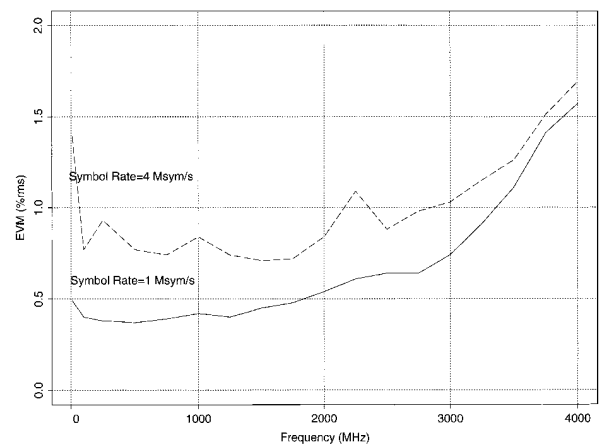
RF EVM performance versus frequency (root Nyquist filter, a = 0.25 , ALC = off, modulation = \pi/4 DQPSK)
