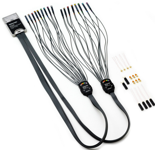
P6780 Differential Logic probes provide high-bandwidth connections for up to 16 digital signals.
