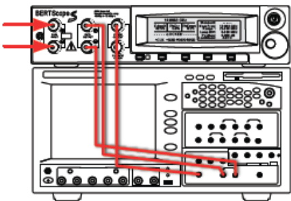
Connecting the BERTScope CR clock recovery instrument to a BERT
