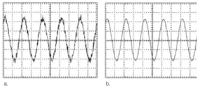
Figure 6.12a and Figure 6.12b. A noisy signal (a) can be cleaned up by a signal averaging (b).
