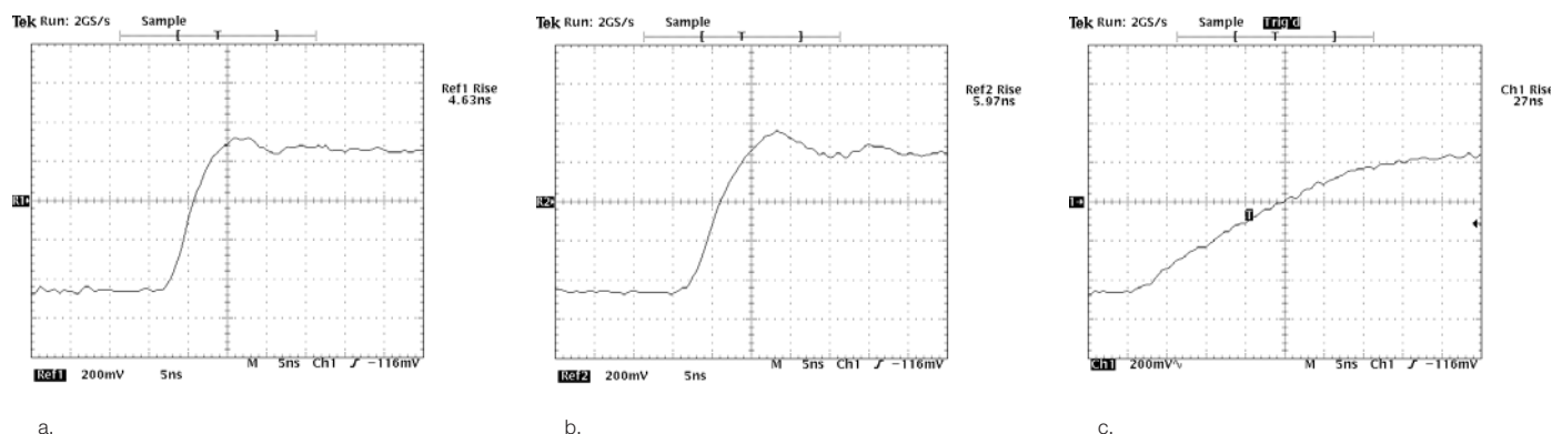
Figure 4.9. Effects on rise time of three different probes: (a) 400 MHz, 10X probe, (b) 100 MHz, 10X probe, and (c) 10 MHz, 1X probe. All measurements were made with the same 400 MHz oscilloscope.
