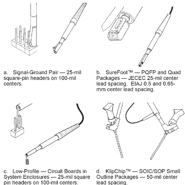
Figure 2.16. Some examples of probe tip adapters for small geometry probes. Such adapters make probing of small circuitry significantly easier and can enhance measurement accuracy by providing high integrity probe to test point connections.
