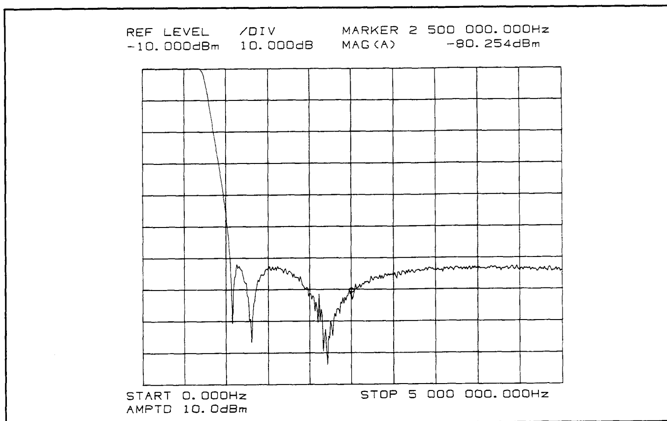
Figure 5-2. Typical Filter Response from 0 to 5 MHz
