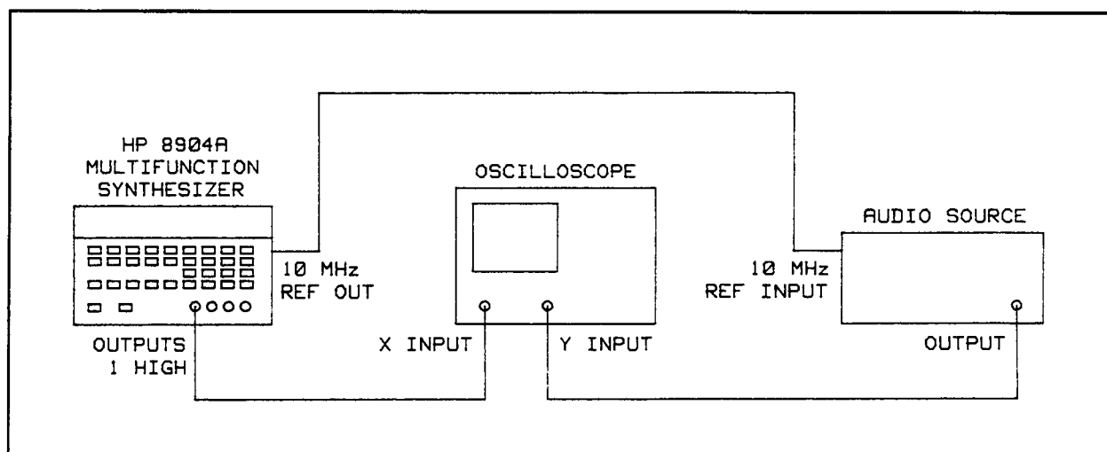
Figure 4-3. Phase Accuracy Performance Test Setup
