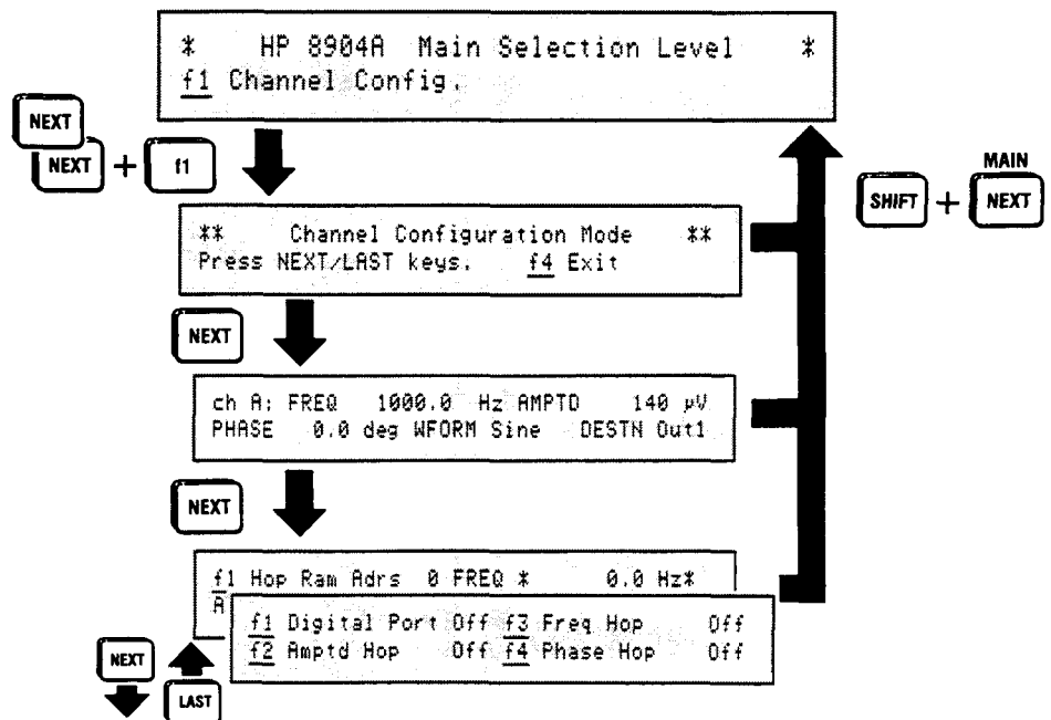
Figure 5-1. How to Access Hop Mode Operation.
