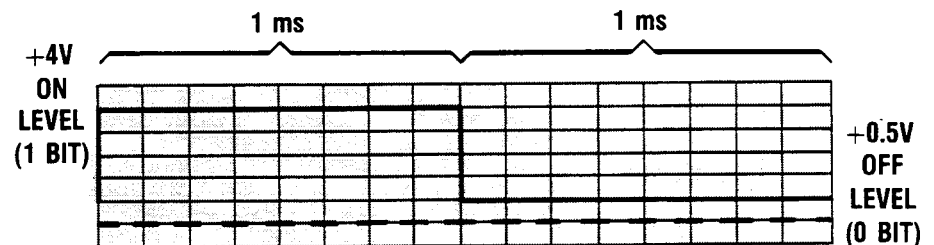
Figure 3-8. 1 and 0 Bit Characteristics.
