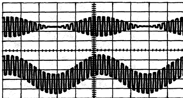
Figure 4-3. Two 20 kHz Square Wave Signals, One Modulated by 1 kHz (top), and the Other Summed with 1 kHz (bottom).
