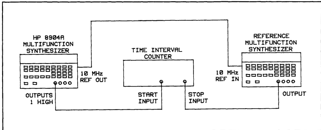
Figure 4-4. Phase Accuracy Performance Test Setup
