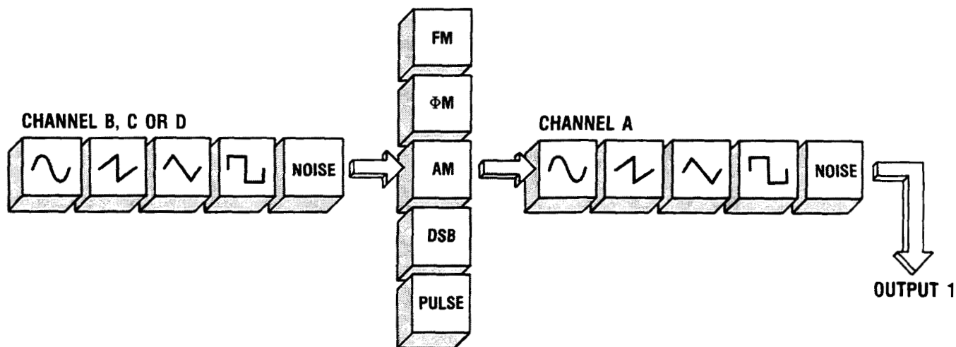
Figure 2-2. The HP 8904A Offers a Wide Selection of Modulation Possibilities.
