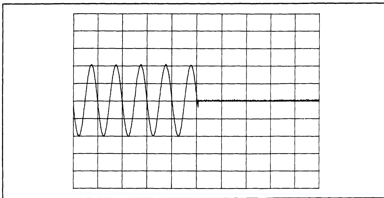
Figure 4-8. Tone Burst Waveform with Slight Negative Slewing
