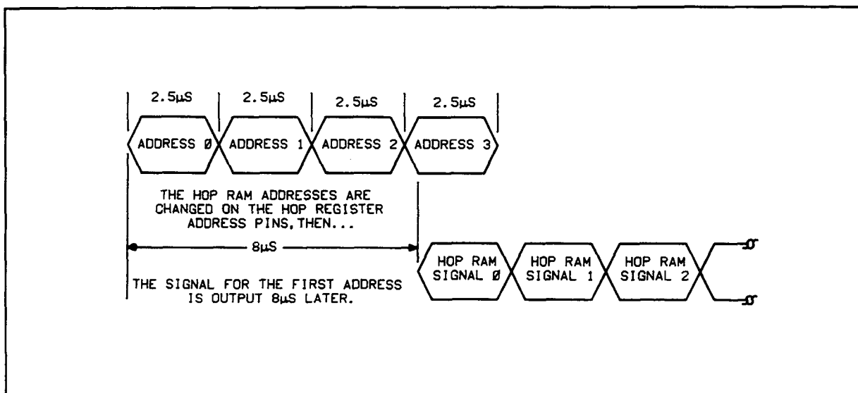
Figure 3-7. Fast Hop Timing Diagram
