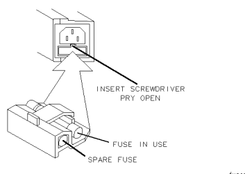
Figure 2-2. Line Fuse Removal and Replacement
