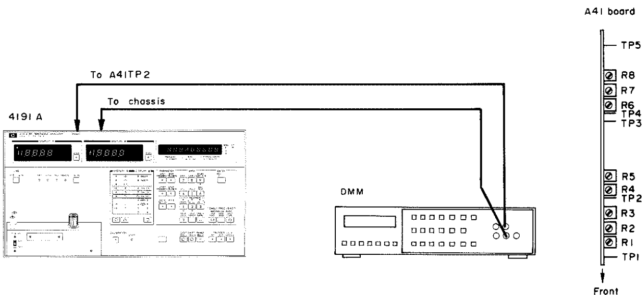
Figure 5-12. Opt. 004 Analog Recorder Output Adjustment Setup.
