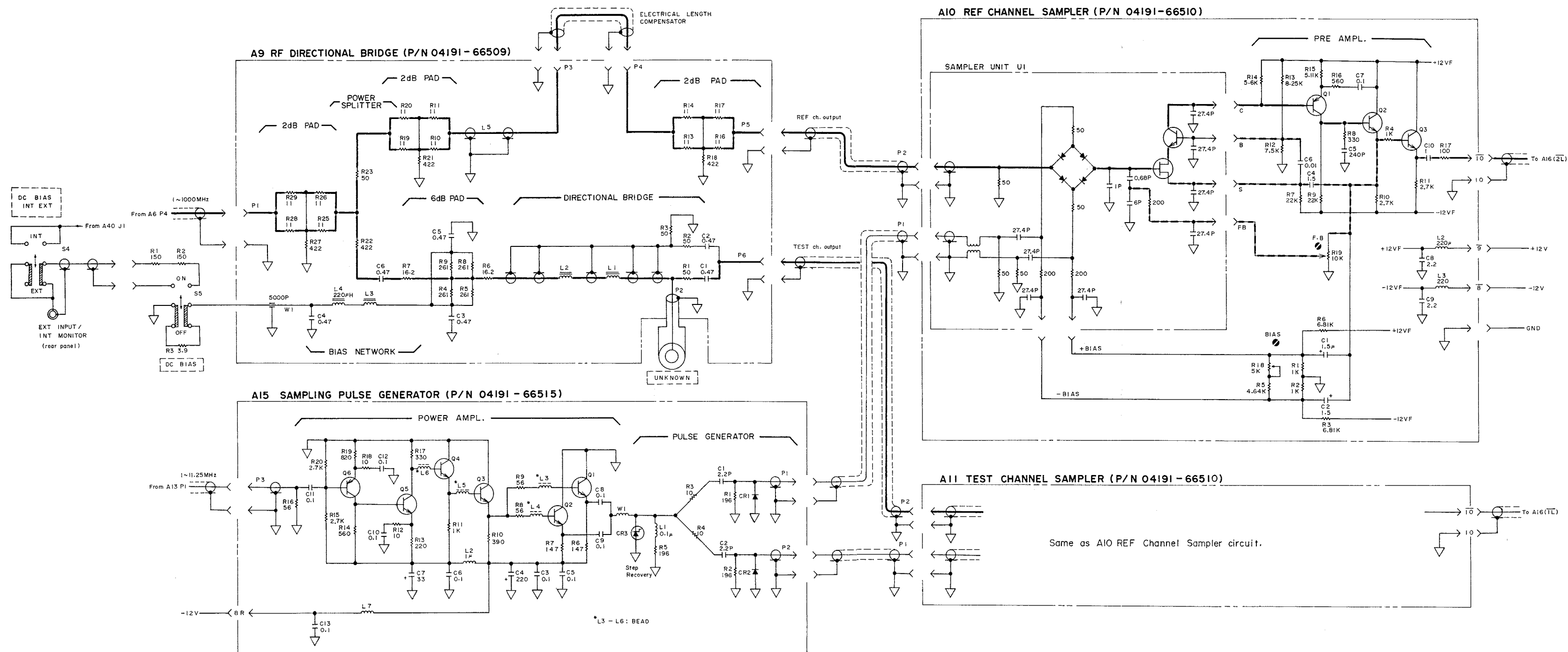
Figure 8-50. A9 RF Directional Bridge, A10 Ref. Channel Sampler, A11 Test Channel Sampler and A15 Sampling Pulse Generator Board Assembly Schematic Diagram.
