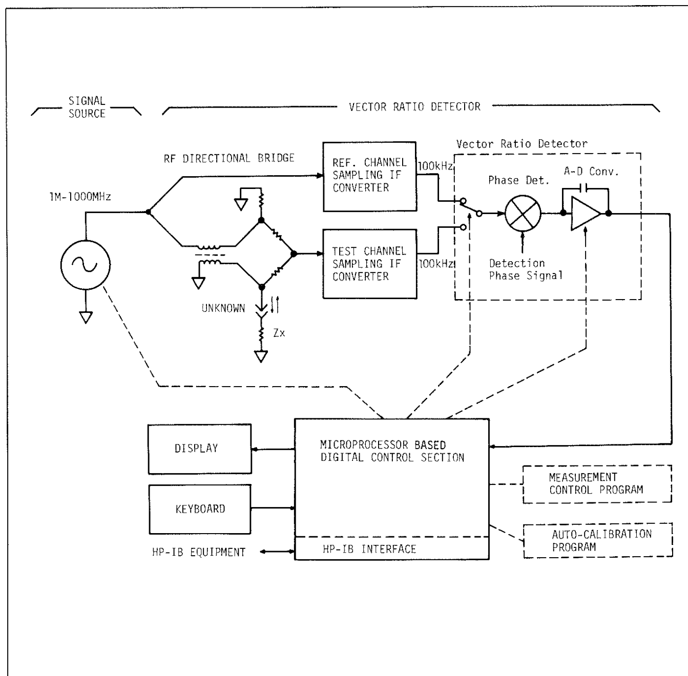
Figure 8-1. 4191A Block Diagram.
