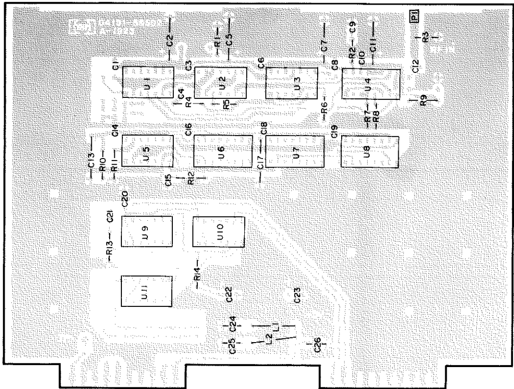
Figure 8-31. A2 100KHz Step Programmable Divider Board Assembly Component Locations.
