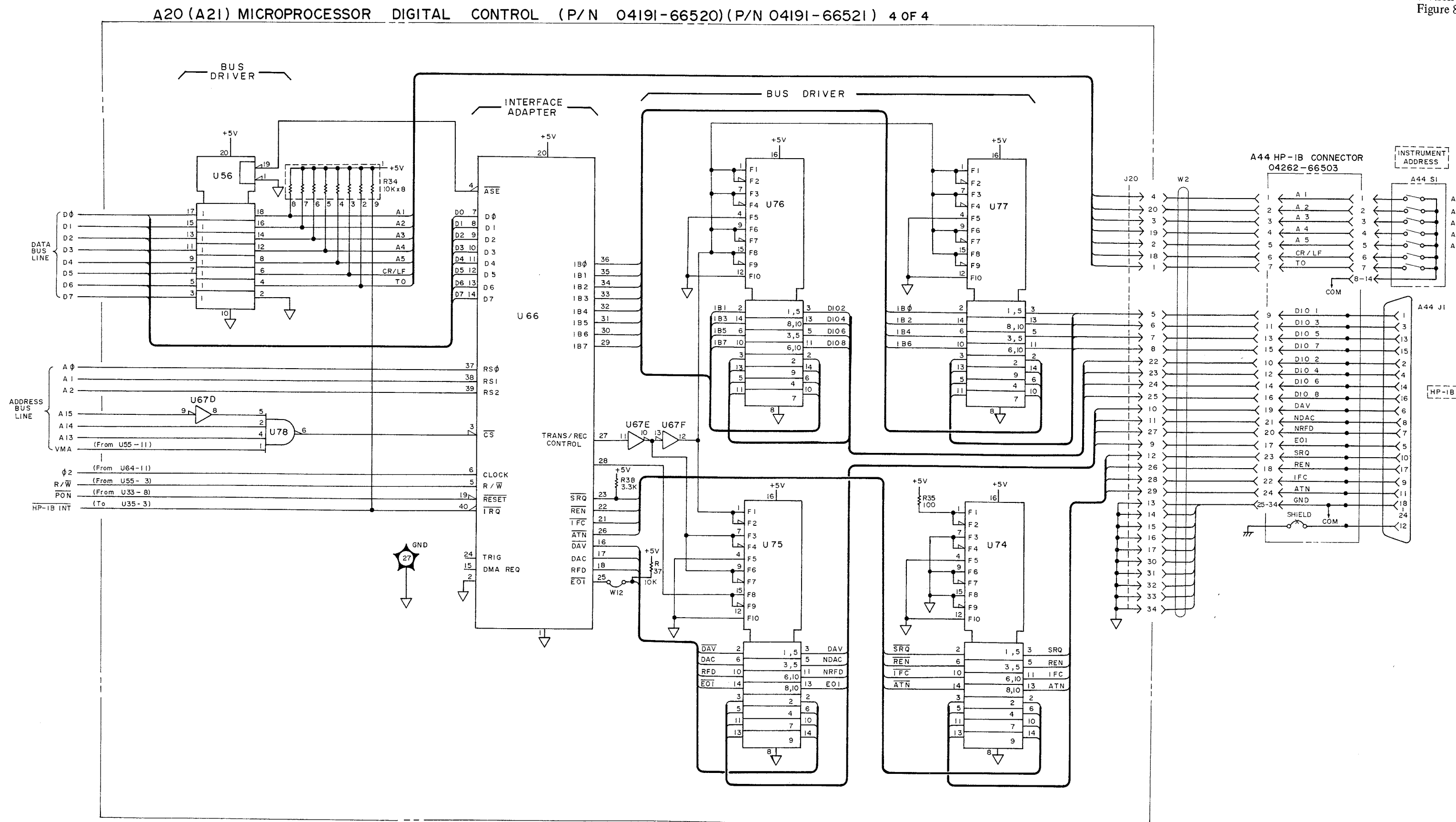
Figure 8-74. A20 (A21) Microprocessor Digital Control Board Assembly Schematic Diagram (sheet 4 of 4).
