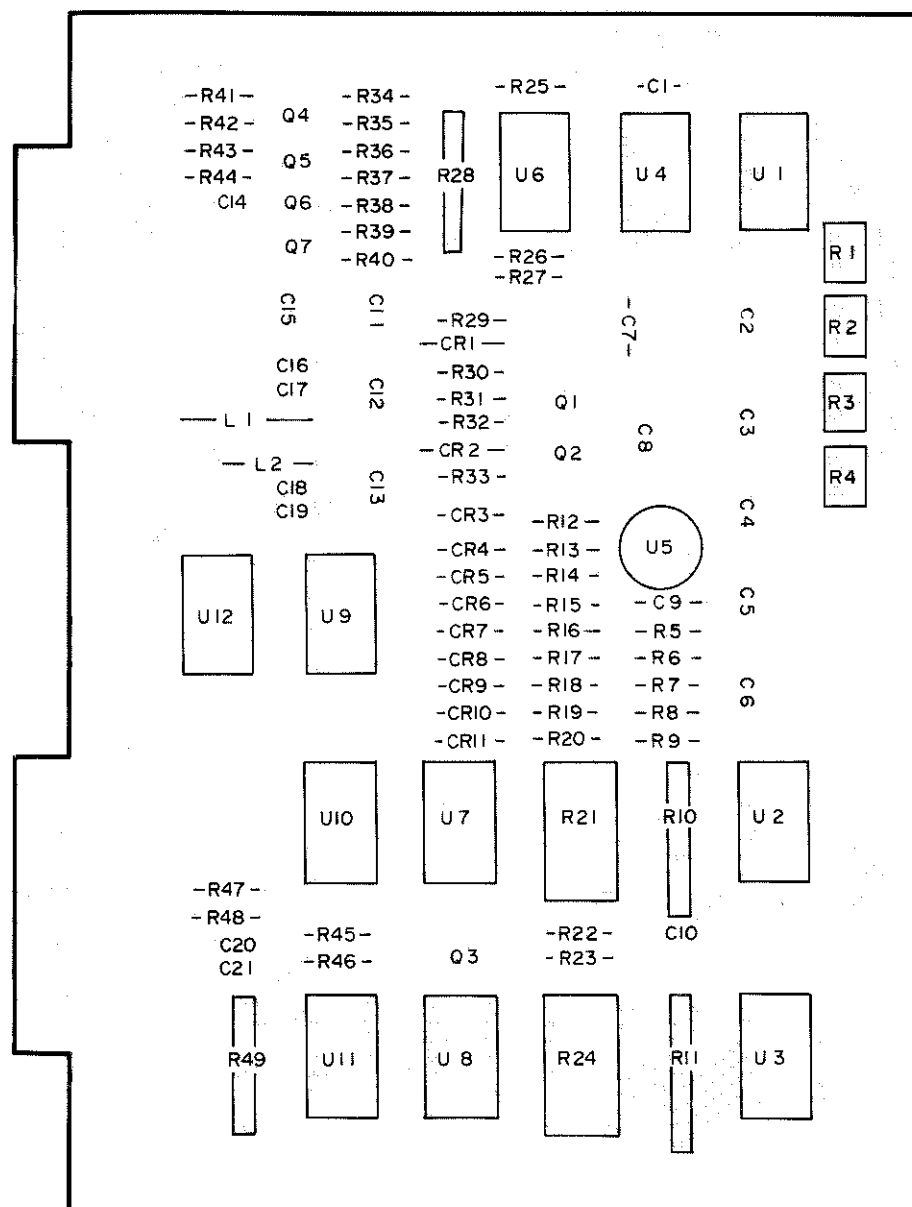
Figure 8-35. A4 Programmable Switch Control Driver Board Assembly Component Locations.
