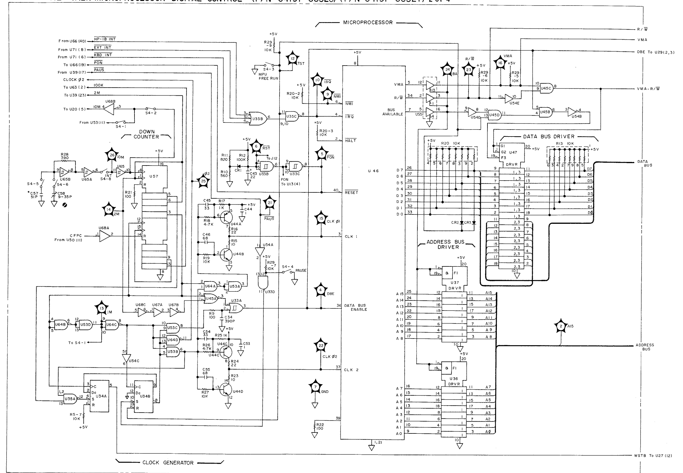
A20 (A21) MICROPROCESSOR DIGITAL CONTROL (P/N 04191-66520) (P/N 04191-66521) 2 OF 4
