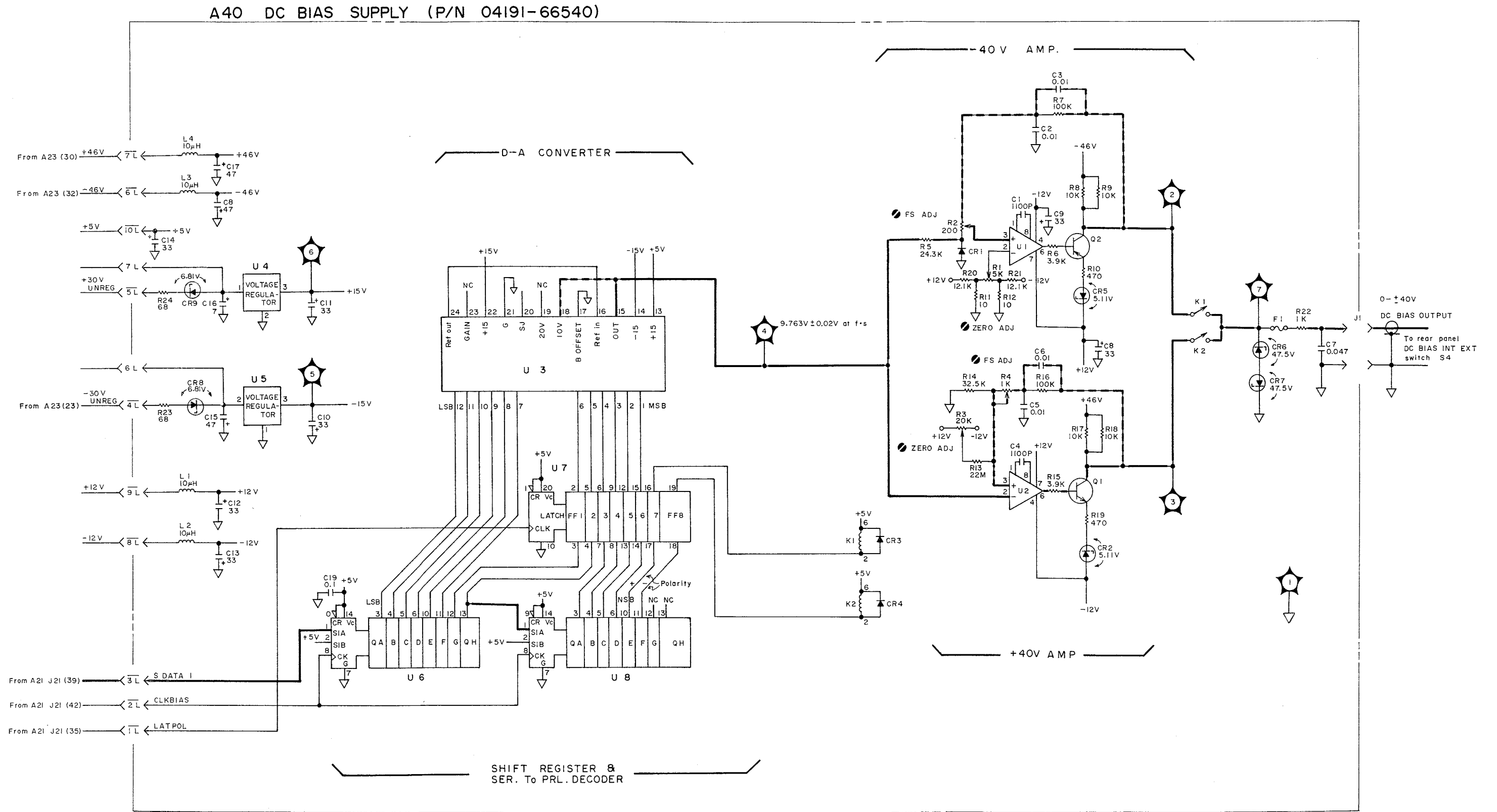
Figure 8-95. A40 DC Bias Supply Board Assembly Schematic Diagram.
