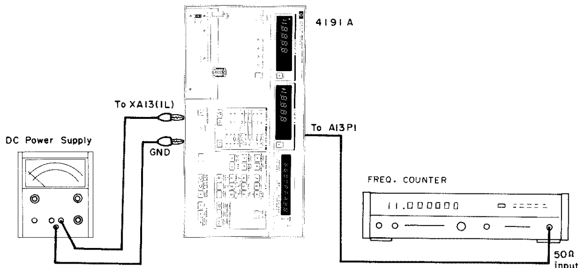
Figure 5-7. Sampling Frequency VTO Adjustment Setup.
