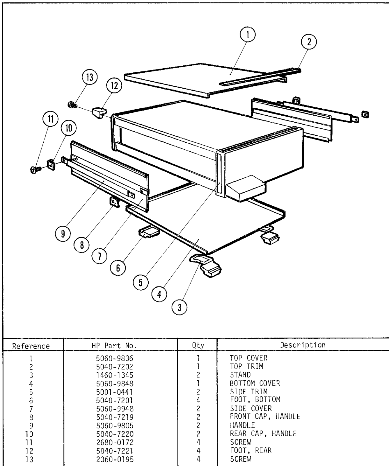
Figure 6-4. Major Mechanical Parts on the Instrument Exterior — Exploded View.
