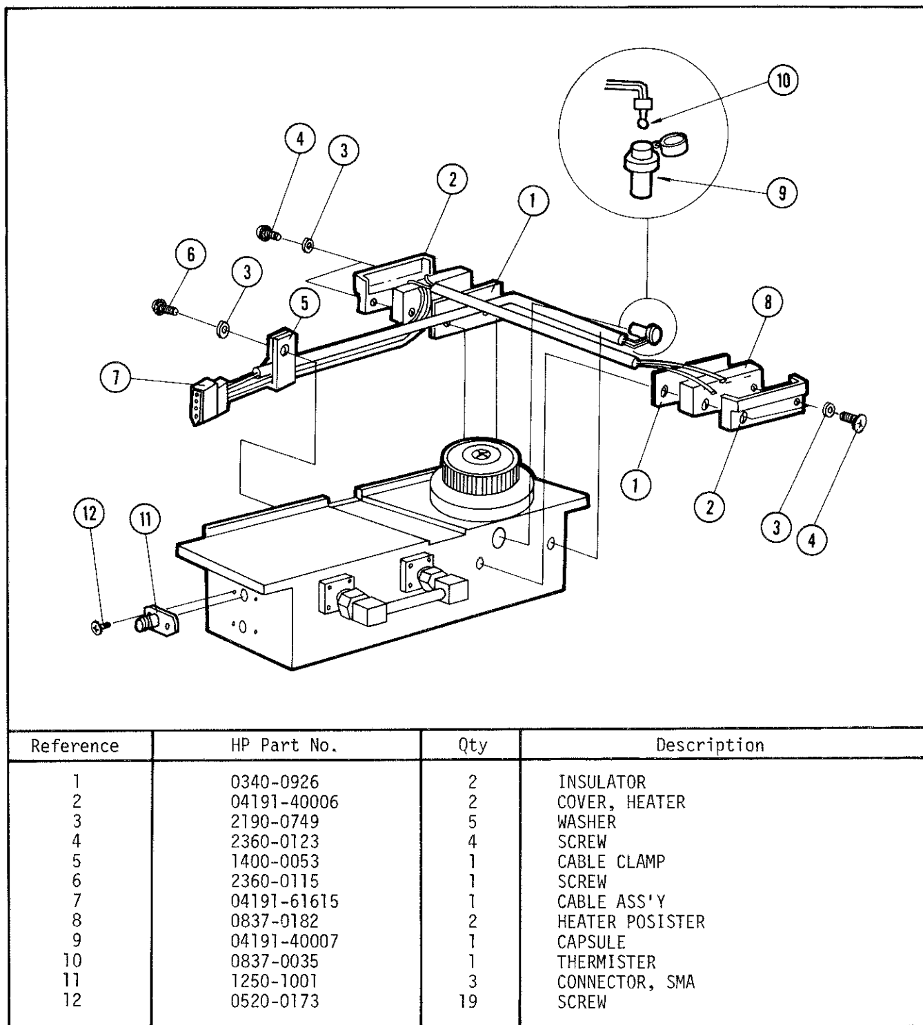
Figure 6-1. Electrical and Mechanical Parts of the Directional Bridge Assembly — Exploded View (sheet 1 of 2).
