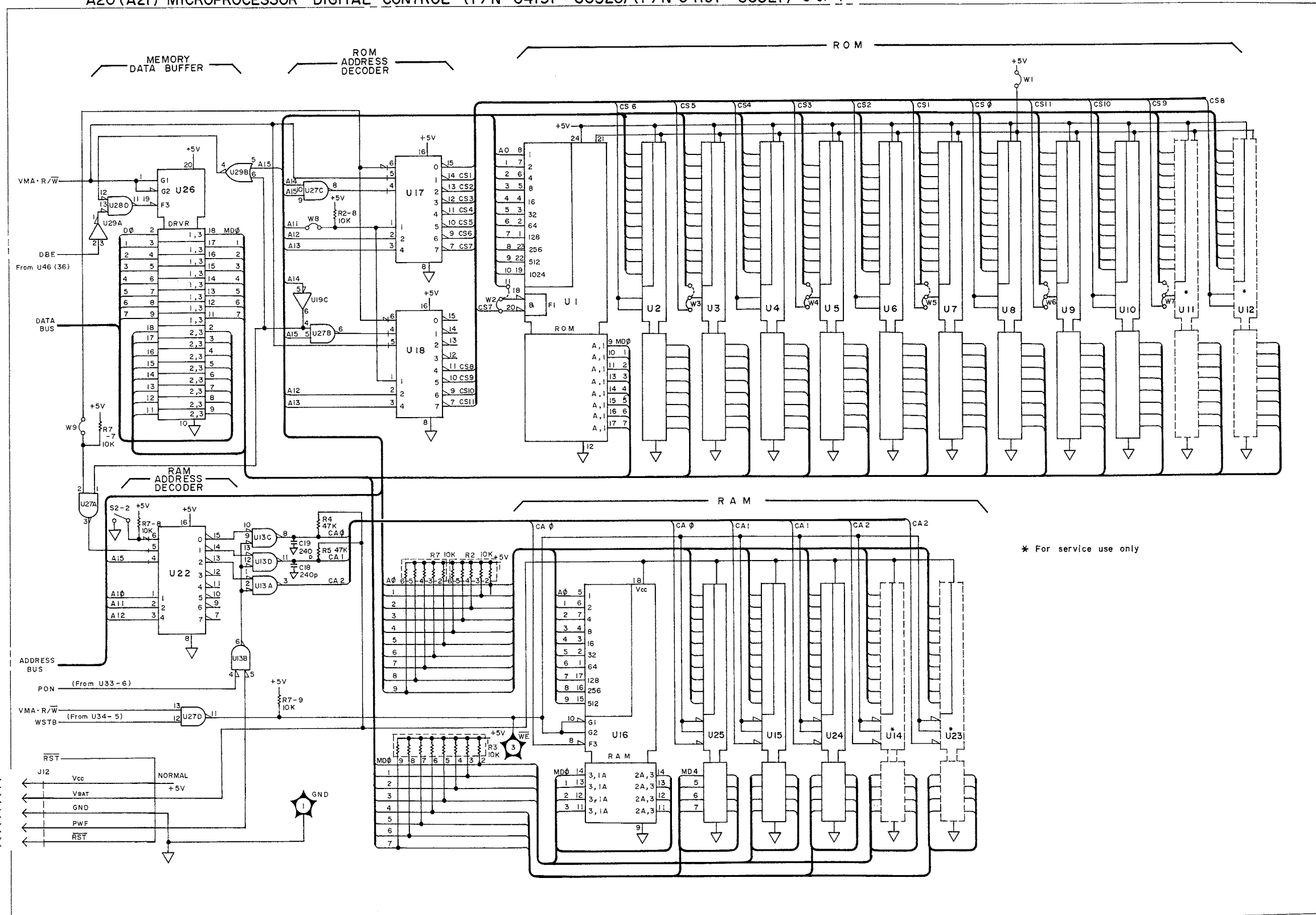
A20 (A21) MICROPROCESSOR DIGITAL CONTROL (P/N 04191 - 66520) (P/N 04191 - 66521) 3 OF 4
