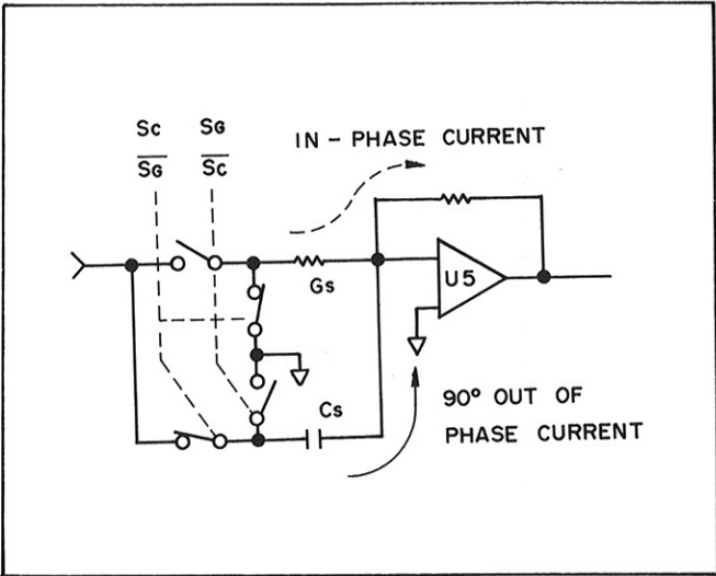
Figure 8-62. C_S/G_S Circuit Simplified Circuit Diagram.
