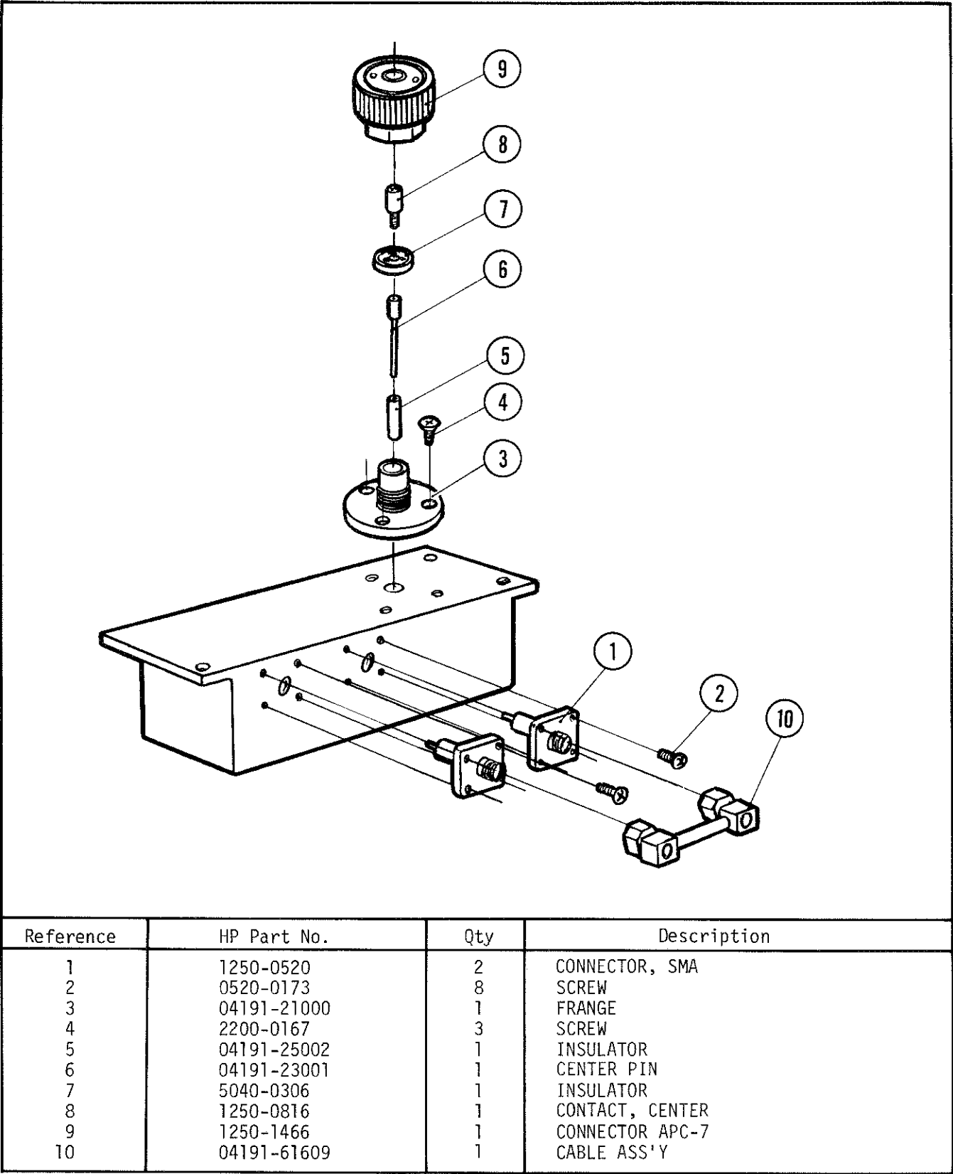
Figure 6-2. Electrical and Mechanical Parts of the Directional Bridge Assembly – Exploded View (sheet 2 of 2).
