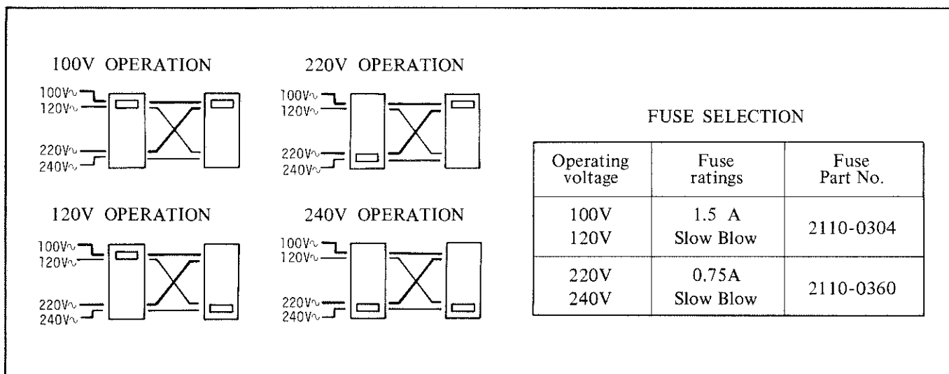
Figure 2-1. Line Voltage and Fuse Selection.
