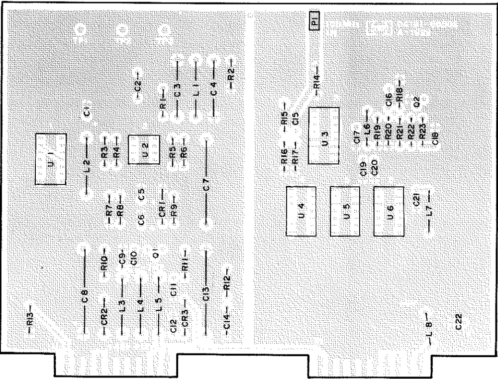
Figure 8-32. A3 Synthesizer Phase Detector Board Assembly Component Locations.
