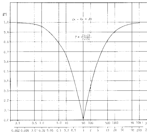
Figure 3-10. Relationship of Reflection Coefficient to Impedance.
