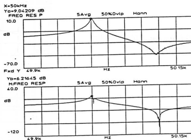
Figure 15-12. Real Part
