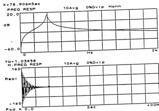
Figure 15-17. Inverse FFT
