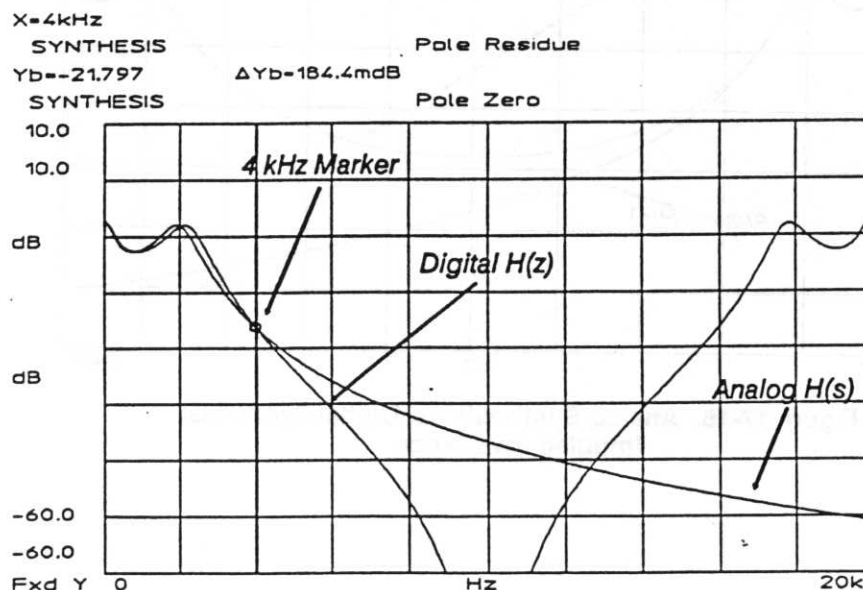
Figure 17-17. Analog Synthesis vs. Digital Synthesis: Bilinear Transformation
