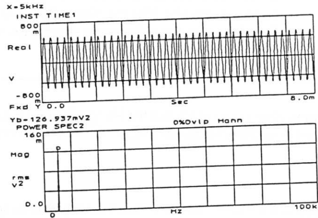
Figure 15-16. FFT
