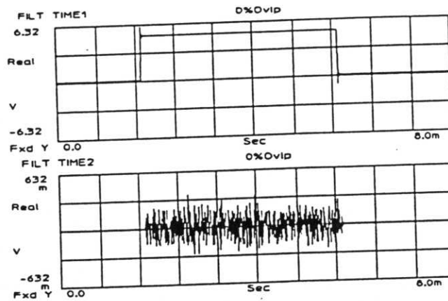
Figure A-3. The SYNC OUT Signal
